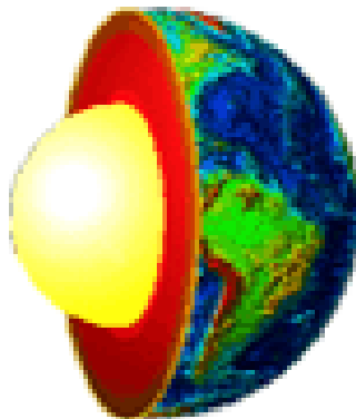
Fig. 1: The Lithosphere
