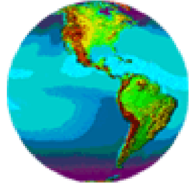
Fig. 2: The Hydrosphere
